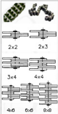
Leaf Chain
